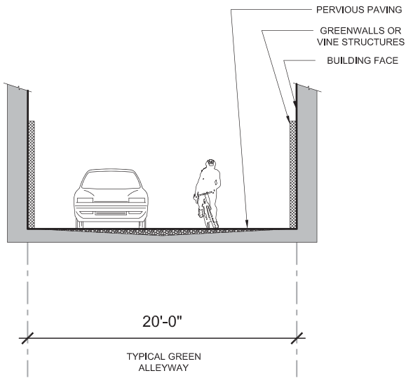
619 CORAOPOLIS BORO. - TYPICAL ALLEYWAY BETWEEN 4TH & 5TH AVENUE (PROPOSED) SCALE: 1"=10'
